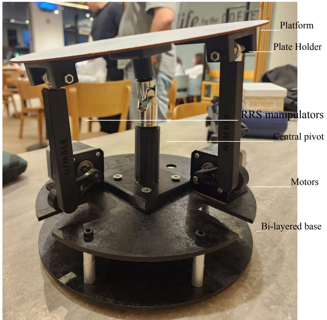
Hardware with key components labelled
